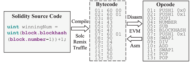
Fig. 1. The relationships among source code, bytecode and opcode.
