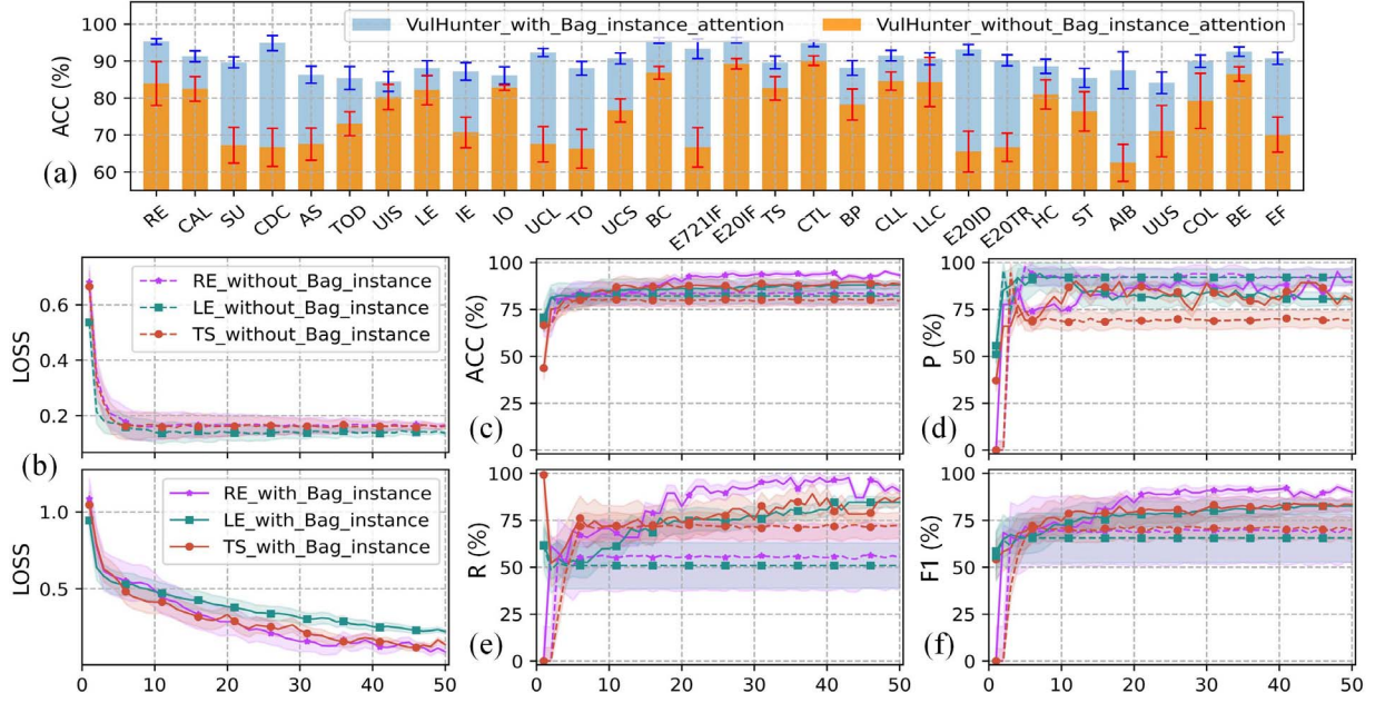
Fig. 10. Performance comparison of VulHunter with and without Bag-instance hybrid attention on Dataset_1 (benign:vulnerable=2:1).
