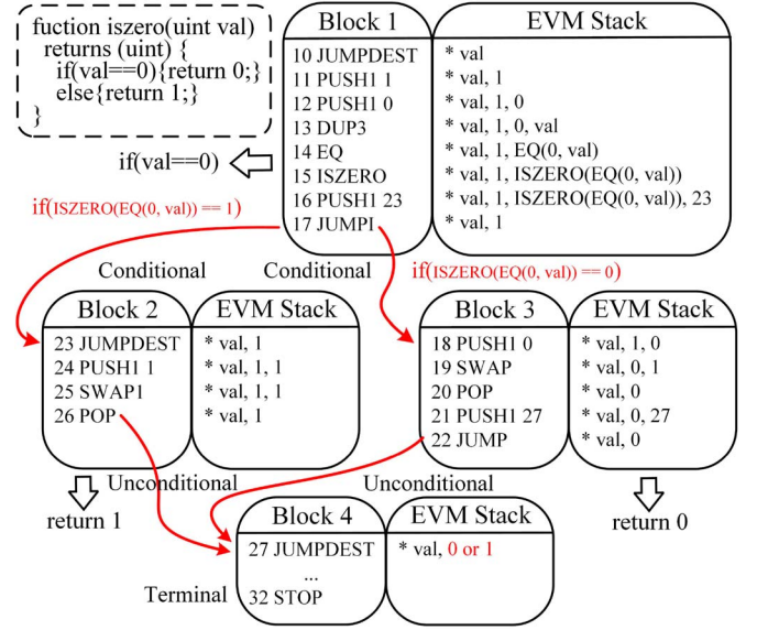
Fig. 4. Example of symbolic reasoning by the CFG Builder.
